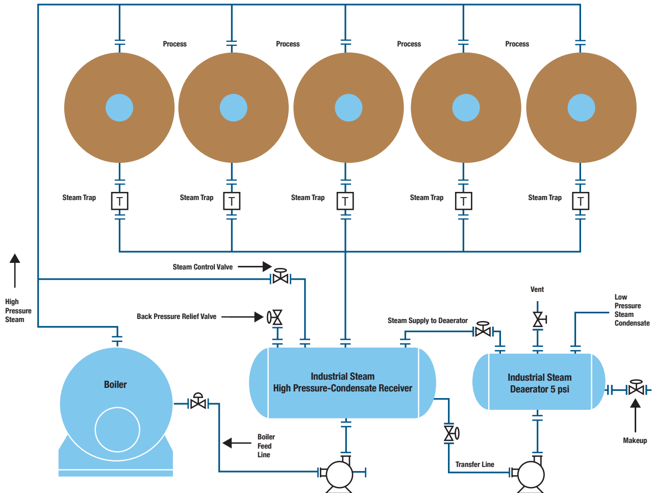
High Pressure Condensate System
