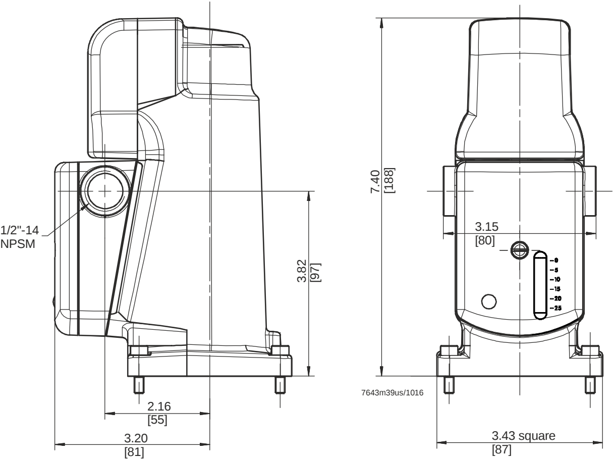
Figure 12. SKP15.xxxUx dimensions
