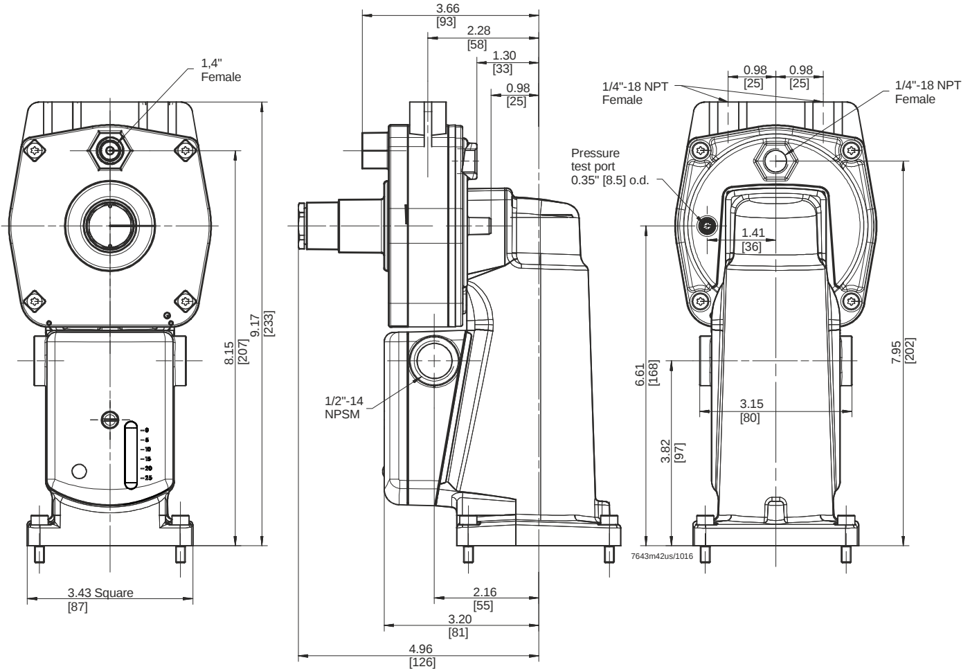
Figure 15. SKP55.xxxUx dimensions
