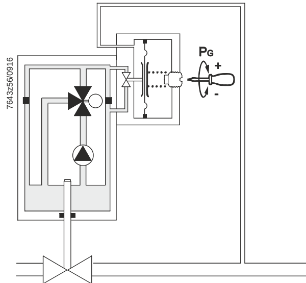
Figure 2. SKP25.xxxUx operation
