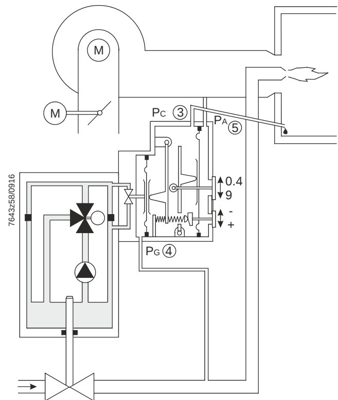
Figure 4. SKP75.xxxUx operation
