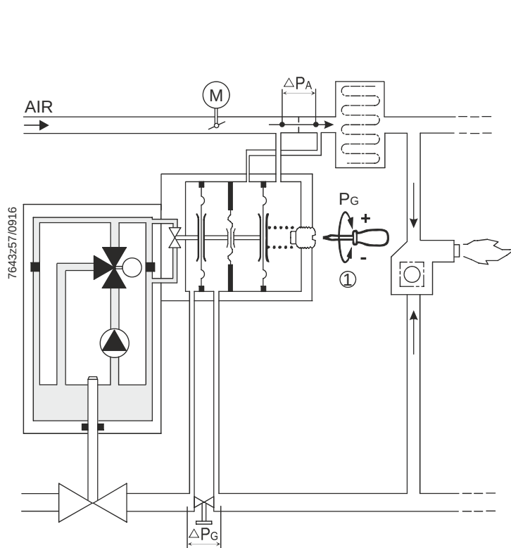
Figure 3. SKP55.xxxUx operation
