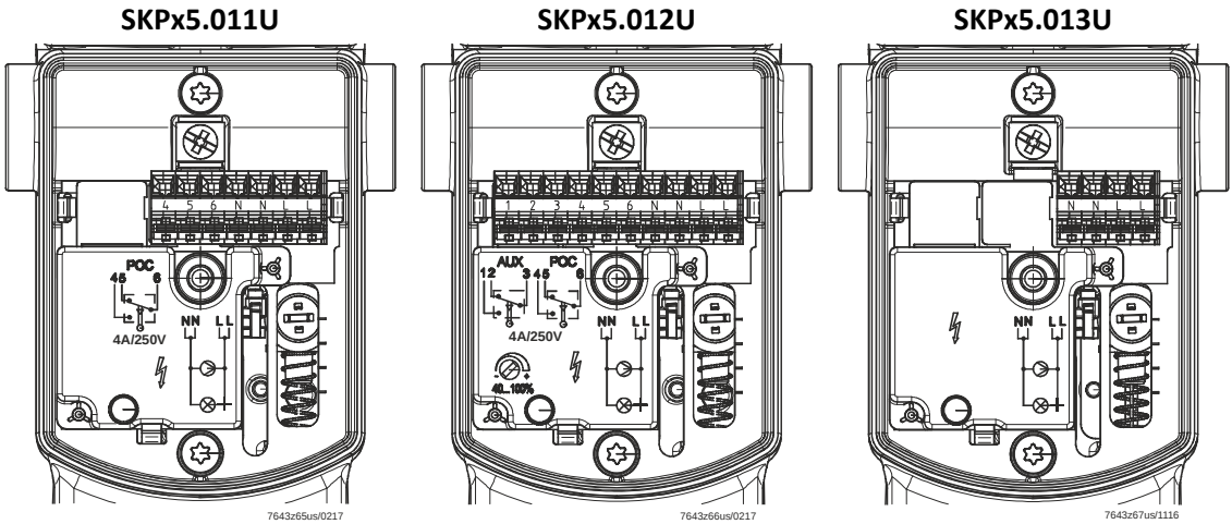
Figure 11. Terminal designations
