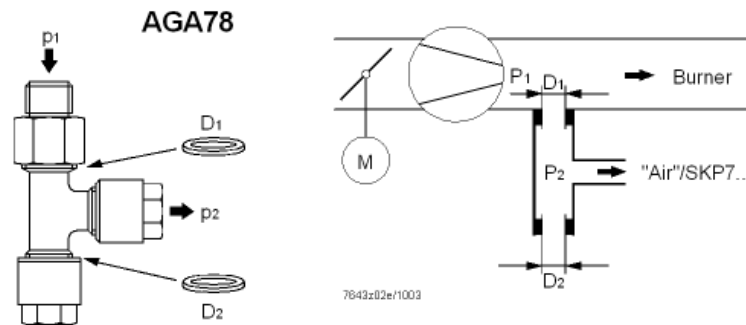
Figure 9. AGA78 Operation.
