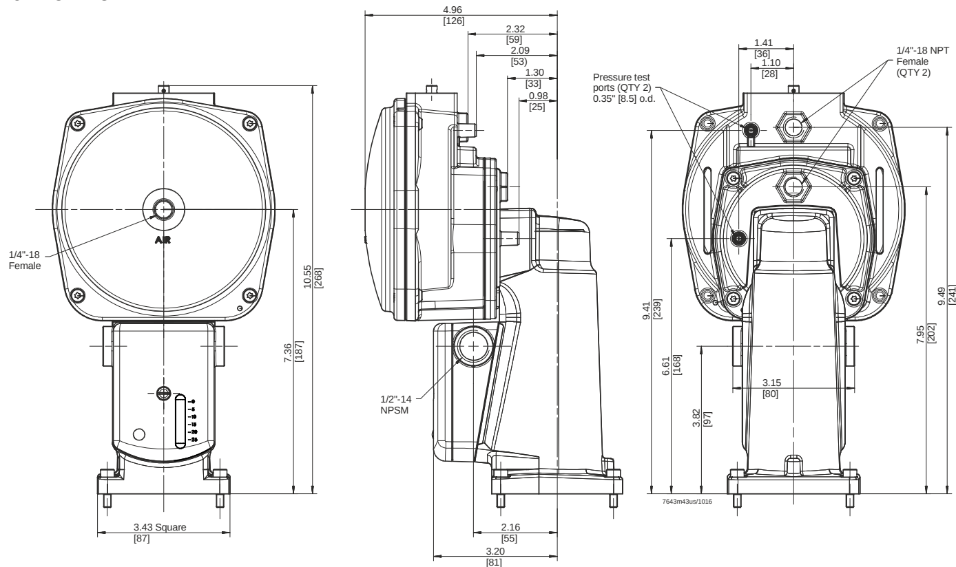
Figure 16. SKP75.xxxUx dimensions
