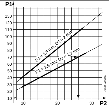
Figure 10. AGA78 Adjustments.
