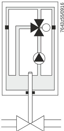
Figure 1. SKP15.xxxUx operation
